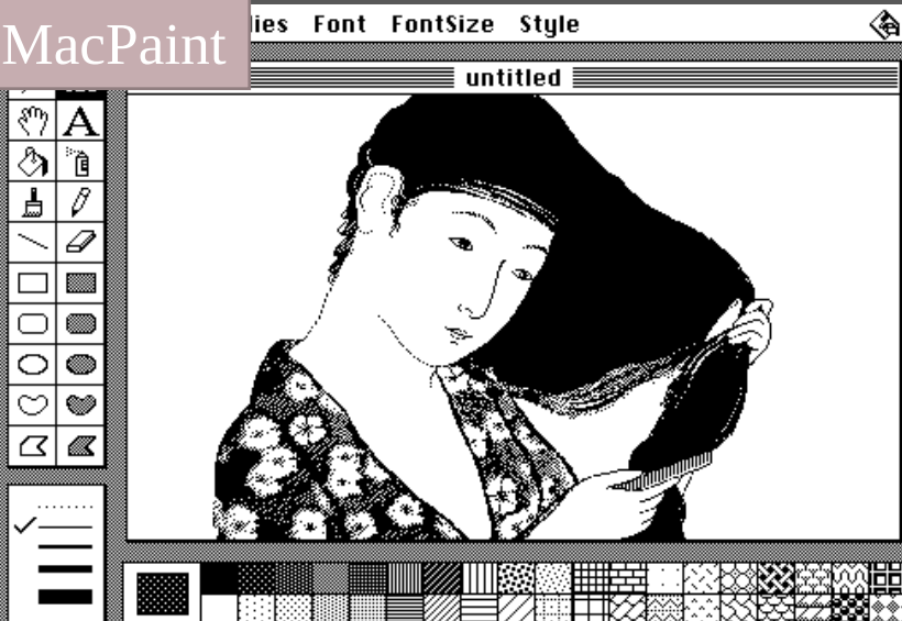
SuperPaint
