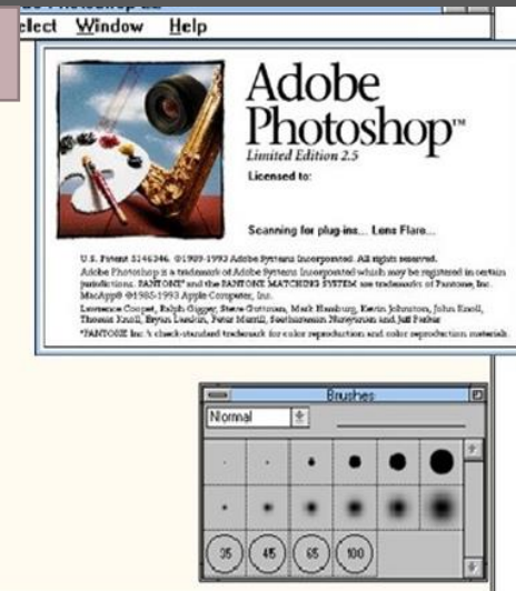
Adobe Photoshop
